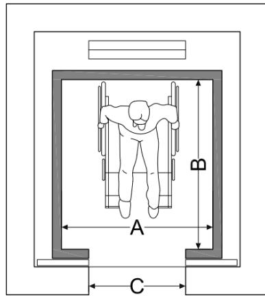
Min. dimensions of disabled accessible Lift
